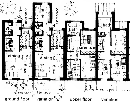
3 Terraced houses with varying depths
